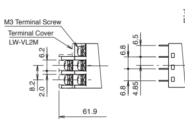
Screw Terminal PC Board Terminal
