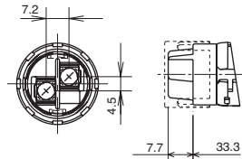
Screw Terminal
